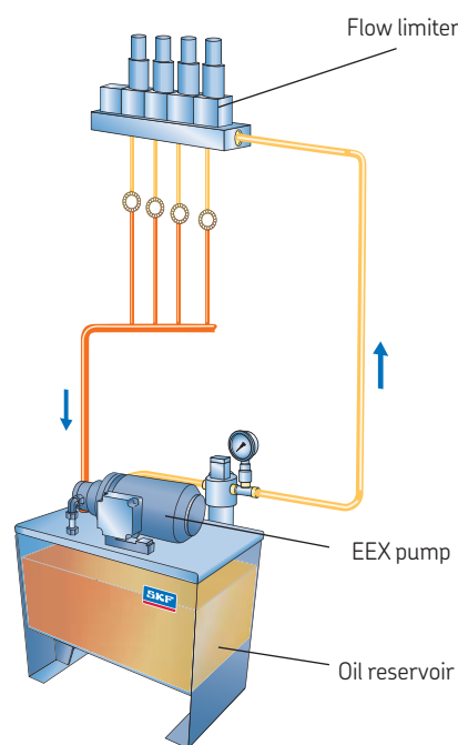
Typical layout of an oil-circulation system
