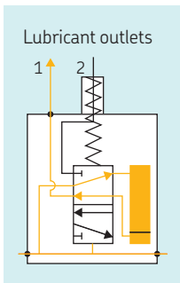
Hydraulic schematic SLC1
