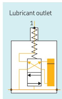
Hydraulic schematic SLC2
