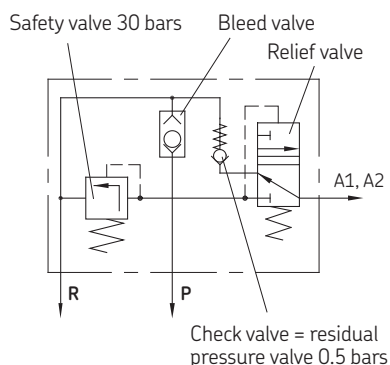
Relief valve circuit diagram
